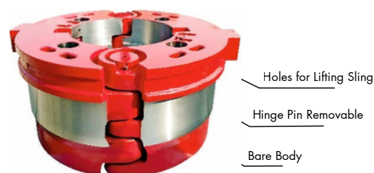
Master Bushing for National RT Model: SDTIMB 3750 Figure No. 1
